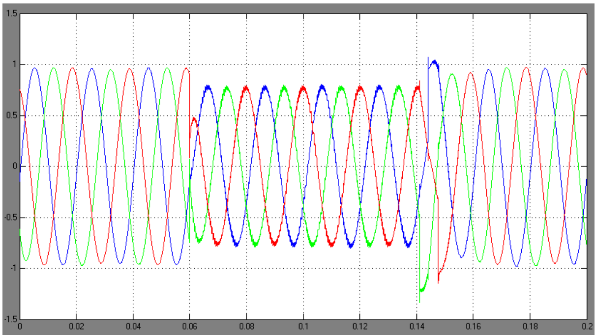
Fig 6. Voltage waveform after compensation with Hysteresis based PI Controller
