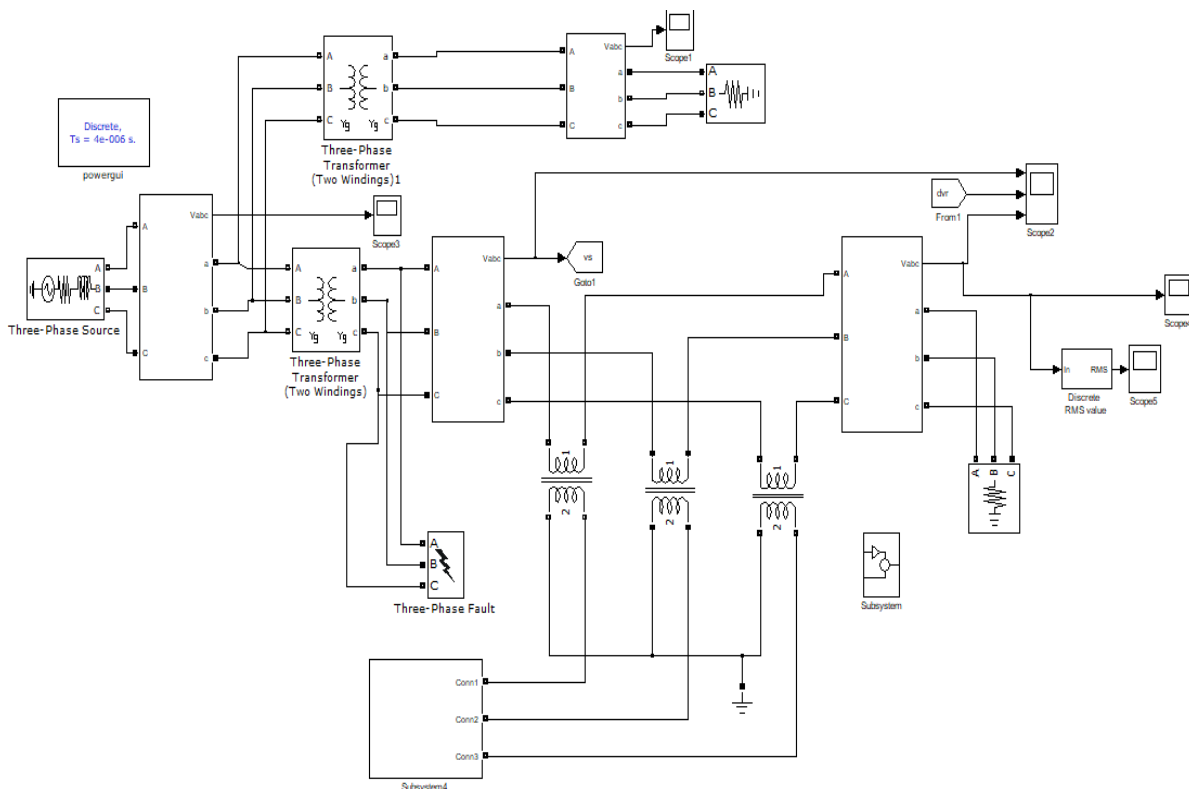
Fig 4. Simulation model of Compensated Transmission line
