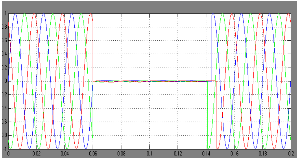
Fig 3. Voltage Across Inductive Load in Uncompensated Line
