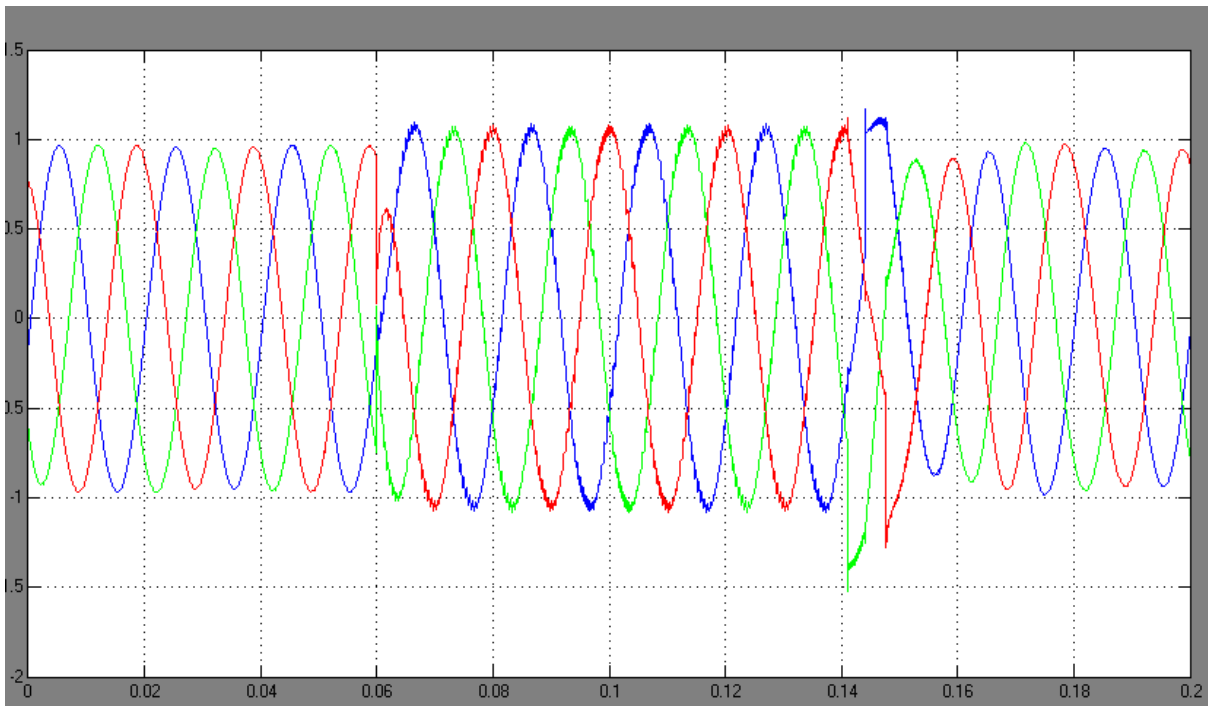
Fig 8. Voltage waveform after compensation with Hysteresis based PID Controller
